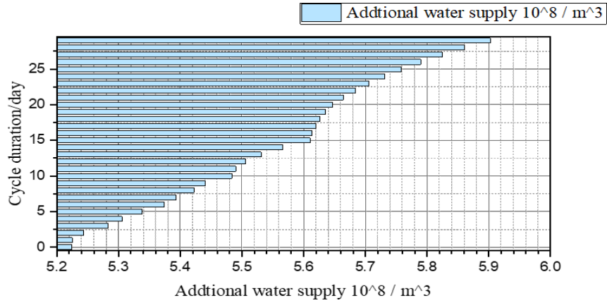
Figure 6: Variation curve of water consumption with water addition cycle
